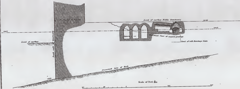
SECTION PARALLEL TO THE SANCTUARY WALL, THROUGH CISTERN XIX & XX. Showing the remains of an ancient passage
